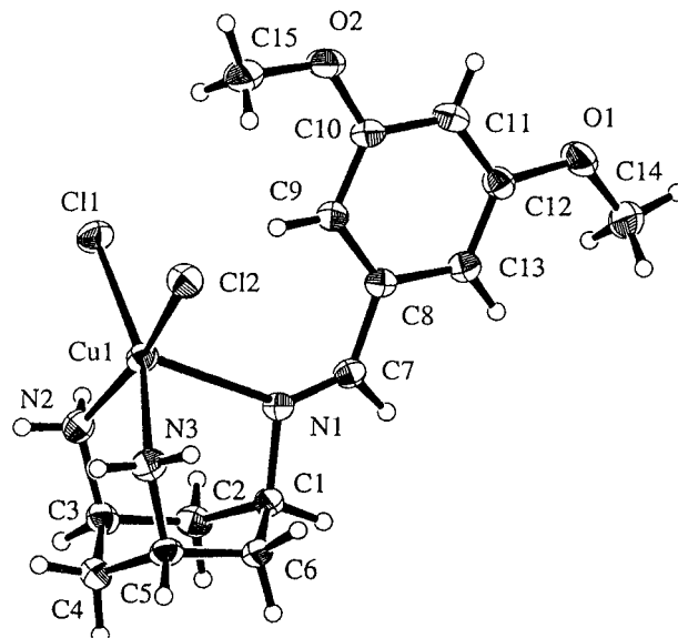
Figure 5. ORTEP 23 representation (30% probability thermal ellipsoids) of 9 .
