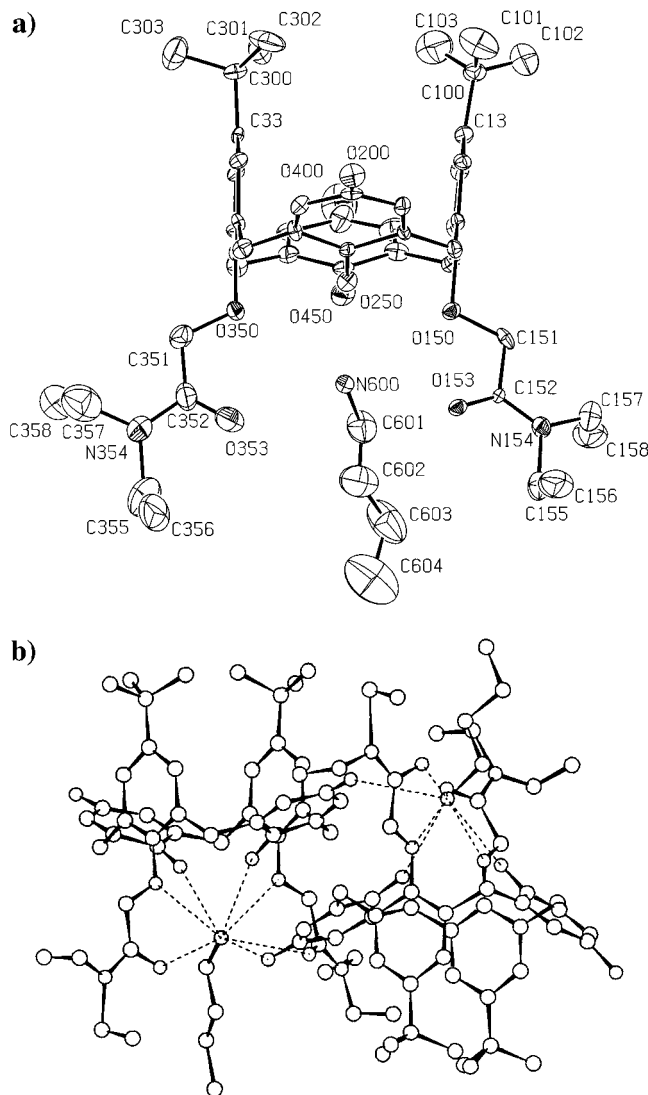
Figure 8. Structure of 4- n - \text{BuNH}_3\text{BF}_4 (a), which forms dimeric units in the crystal (b). Thermal ellipsoids are shown at the 15% probability level.
