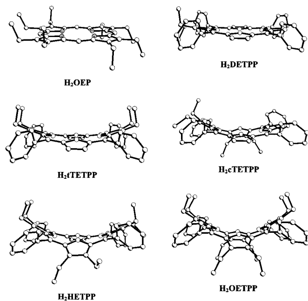
Figure 1. Side views of the molecular structures of H 2 OEP, H 2 DETTP, H 2 tTETTP, H 2 cTETTP, H 2 HETTP, and H 2 OETTP.
