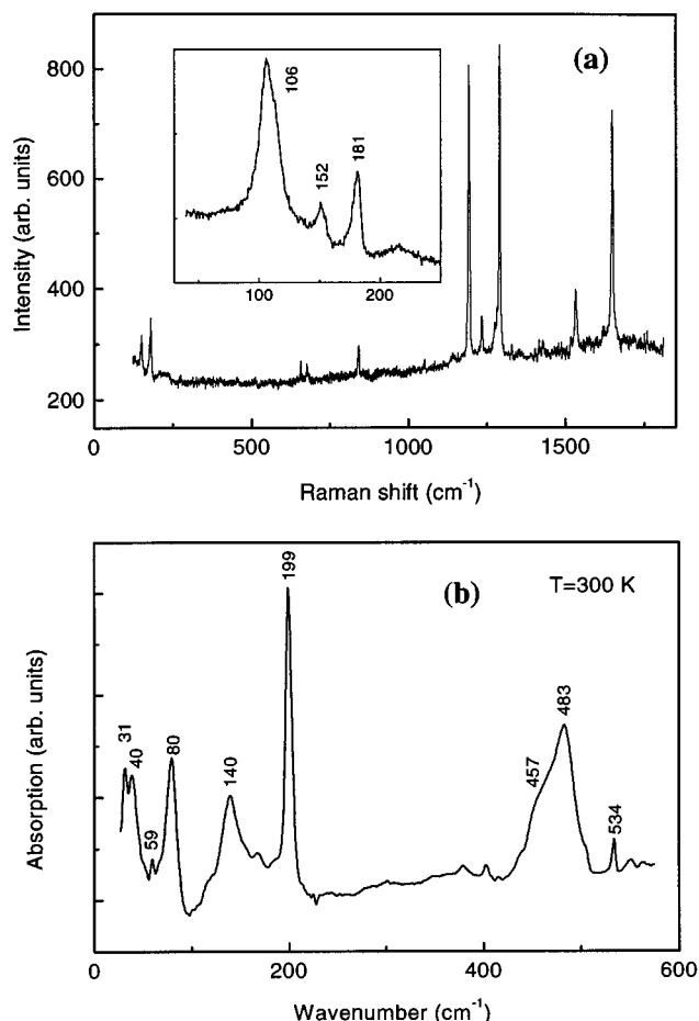
Figure 2. (zz)-polarized Raman scattering spectrum of 1 at T = 300 K and \lambda_{\text{exc}} = 514.5 nm. The inset shows the spectrum of 1 in the range 30–250 \text{cm}^{-1} . (b) Infrared absorption spectrum of 1 at T = 300 K.
