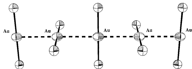
Figure 1. Portion of a single 1D chain of Au 2 − ions in 1 . The dashed lines represent Au(I)–Au(I) aurophilic interactions (Au–Au = 3.3767(3) Å). (Ellipsoids are drawn at 50% probability.)
