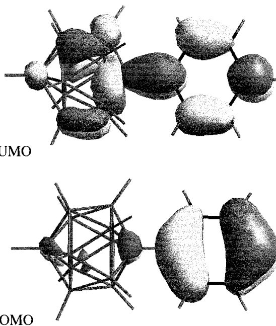
Figure 3. Representation of the HOMO (-9.86 eV; A'') and the LUMO (2.46 eV; A'') of 1c-E .
