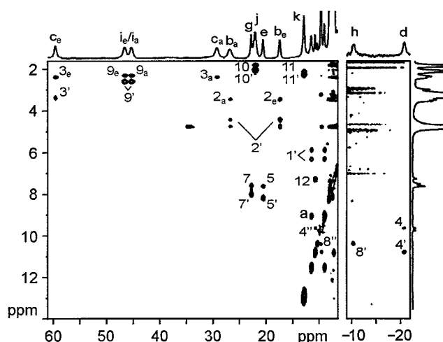
Figure 3. 1 H EXSY spectrum (250 MHz, 298 K, 20 ms mixing time, 133 ms recycle time) of Co(II)- 1 in 2:3 CH 3 OH/CD 3 OD. Labels for the peaks correspond to the structure shown in Figure 1.
