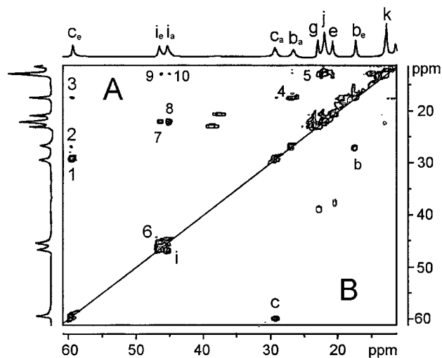
Figure 4. ^1\text{H} TOCSY (A) and EXSY (B) spectra (250 MHz, ambient temperature, 30 and 80 ms mixing time, and 190 and 240 ms recycle time, respectively) of \text{Co(II)-1} in methanol- d_4 . Labels correspond to the structure shown in Figure 1. The cross signals 1, 4, 5, and 7 are also detected in the COSY spectrum of the complex.
