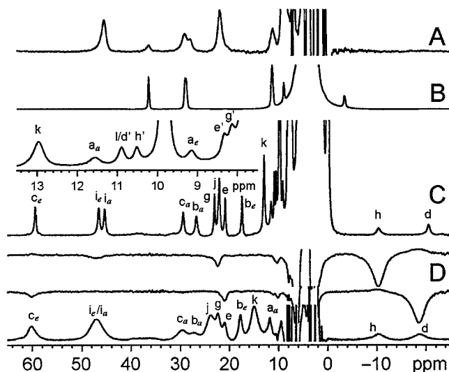
Figure 2. 1 H NMR spectra (250 MHz, 298 K, CD 3 OH) of complexes Co(II)–( 3 ) 2 (A), Co(II)– 3 (B), Co(II)– 1 (C), and Co(II)– 2 (D). The 1D NOE difference spectra in part D are obtained with the signals at –11 ppm (top) and –19 ppm (bottom) saturated for 50 ms. Labels of the signals correspond to the structure shown in Figure 1. Signals d, h, and l are solvent exchangeable and disappear when the complexes are dissolved in methanol- d 4 .
