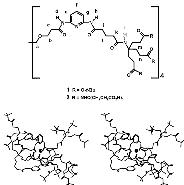
Figure 1. Schematic structure of the 12-ester diamidopyridine dendrimer ( 1 ) and the 36-acid diamidopyridine dendrimer ( 2 ) and the 3D model of the Co(II)– 1 complex constructed with distance constraints from NMR relaxation times by the use of the Cerius 2 molecular modeling program. Hydrogen atoms are omitted, and other atoms are not labeled in the structures for clarity.
