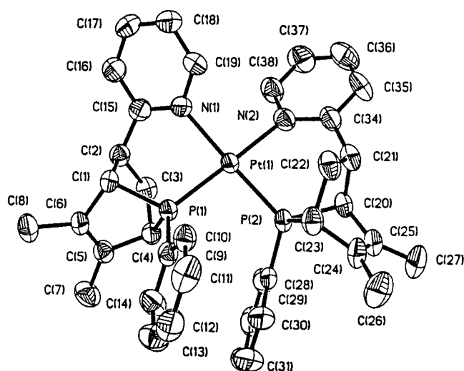
Figure 5. Structural drawing of the cation of 5b , showing the atom-numbering scheme (40% probability ellipsoids). Selected bond distances (Å) and bond angles (deg): Pt(1)–P(1), 2.237(2); Pt(1)–P(2), 2.238(2); Pt(1)–N(1), 2.129(5); Pt(1)–N(2), 2.128(5); P(1)–Pt(1)–P(2), 92.49(6); N(1)–Pt(1)–N(2), 89.8(2); N(2)–Pt(1)–P(1), 88.3(2); N(2)–Pt(1)–P(2), 90.1(2).
