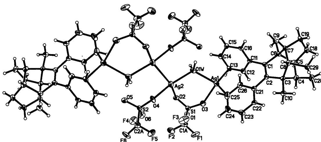
Figure 3. ORTEP diagram of the dimeric [\text{IXAg}(\mu_2\text{-OTf})(\mu_2\text{-H}_2\text{O})\text{OTfAg}\cdots\text{AgOTf}(\mu_2\text{-H}_2\text{O})(\mu_2\text{-OTf})\text{AgIX}] complex with an unusually short \text{Ag}\cdots\text{Ag} contact of 3.234(1) Å. Thermal ellipsoids are shown at the 50% probability level.
