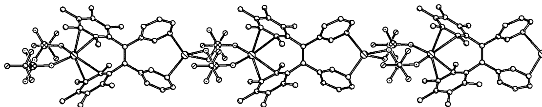
Figure 6. Infinite regular chain formed along 2-fold axis in structure X (AgOTf) 2 . Note the head-to-tail arrangement and \mu_2 bridging function of triflate ligands.
