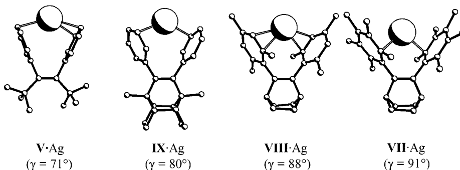
Figure 4. Progressive structural changes in silver(I)/stilbenoid complexes with increasing values of \gamma (left opening between benzene rings). See text and Table 3.
