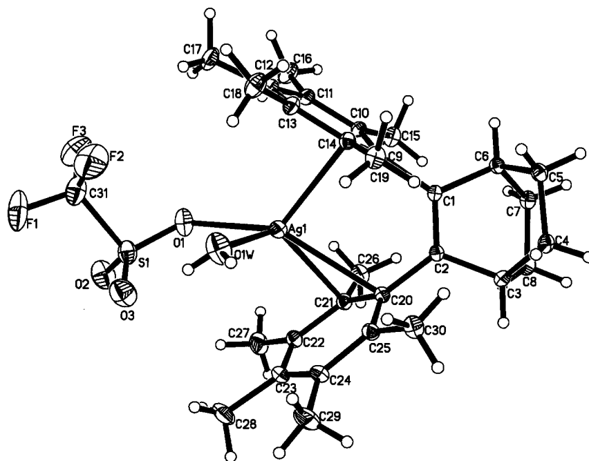
Figure 1. ORTEP diagram of the monomeric [VIIAgOTf(H 2 O)] complex. Thermal ellipsoids are shown at the 50% probability level.
