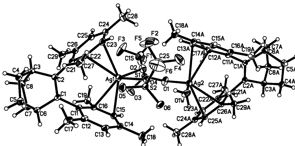
Figure 2. ORTEP diagram of the dimeric [\text{VIIIAgOTf}(\mu_2\text{-OTf})(\text{H}_2\text{O})\text{AgVIII}] complex. Thermal ellipsoids are shown at the 50% probability level.
