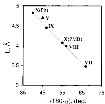
Figure 5. Silver penetration L (see structure XI ) as a function of dihedral angle \alpha between benzene rings (see structure II ). Correlation factor for the linear approximation is R = 0.9995 (Gano's structure V ·Ag was not included in the computation).
