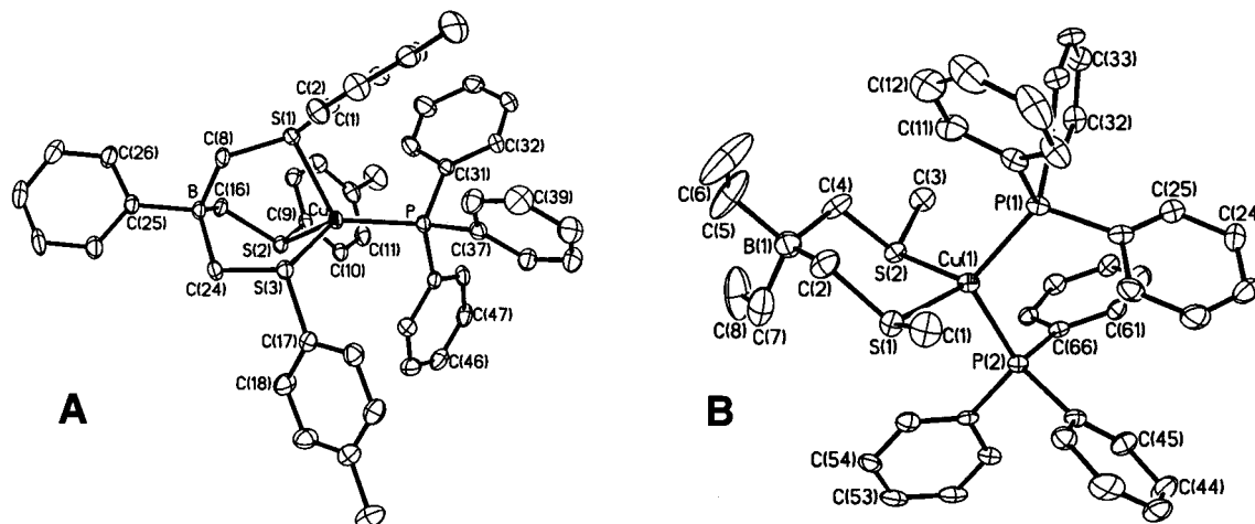
Figure 4. Thermal ellipsoid plots of [\text{PhTt}^{\text{Ph}}]\text{Cu}(\text{PPh}_3) (A) and [\text{Et}_2\text{Bt}]\text{Cu}(\text{PPh}_3)_2 (B) at the 30% probability level; hydrogen atoms are not shown.
