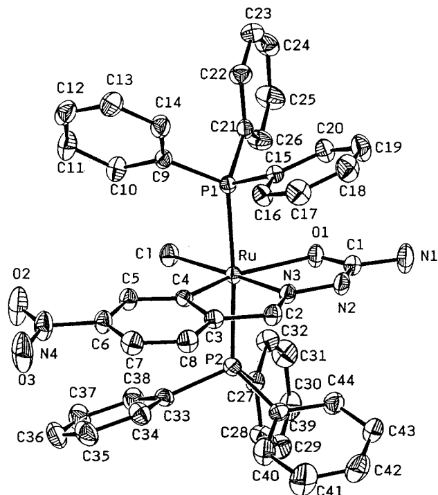
Figure 1. Structure of trans -[Ru(PPh 3 ) 2 (L-NO 2 )Cl].
