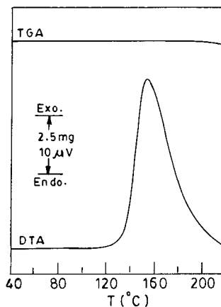
Figure 2. Thermogram of trans -[Ru(PPh 3 ) 2 (L-NO 2 )Cl].
