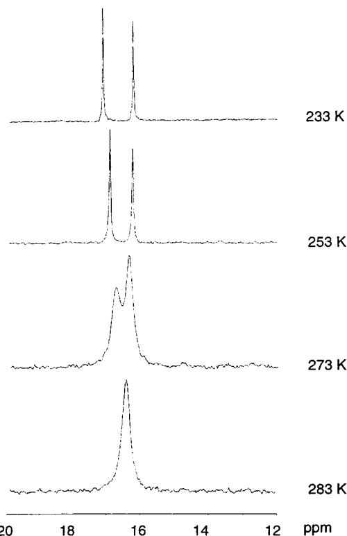
Figure 2. ^{31}\text{P}\{^1\text{H}\} NMR spectra at variable temperature for complex 4 in \text{CDCl}_3 .
