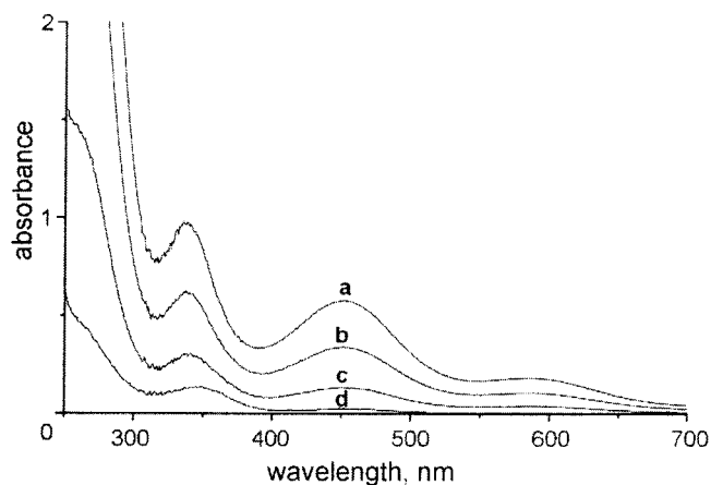
Figure 1. Absorption spectral changes recorded for the reaction of 3 \times 10^{-3} \text{ M } [\text{Fe}^{\text{II}}(\text{H}_2\text{O})_6]^{2+} with NO. Experimental conditions: 0.2 M acetate buffer, pH = 5.0, 25 °C. Curves: trace a, [\text{Fe}^{\text{II}}(\text{H}_2\text{O})_6]^{2+} solution saturated with NO; trace b, a + Ar brief (10 s); trace c, b + Ar brief (10 s); trace d, c + Ar brief (10 s).
