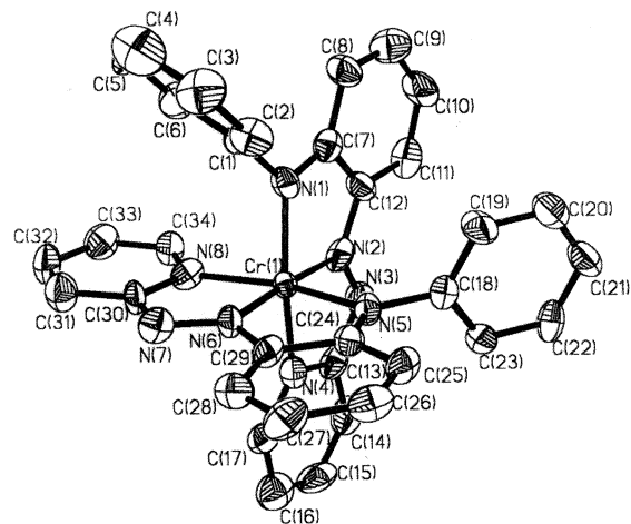
Figure 1. Molecular structure and atom numbering scheme for [\text{Cr}(\text{L}^{1a})_2](\text{ClO}_4) .
