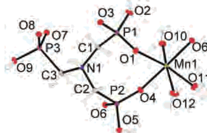
Figure 5. ORTEP drawing of \text{Mn}[\text{HN}(\text{CH}_2\text{PO}_3\text{H})_3(\text{H}_2\text{O})_3] ( 2 ), showing the octahedral coordination of Mn by three water molecules and three phosphonate oxygens. Two phosphonate groups of the same nitrilotris-(methylenephosphonate) bond to the same Mn forming an eight-membered ring through chelation.
