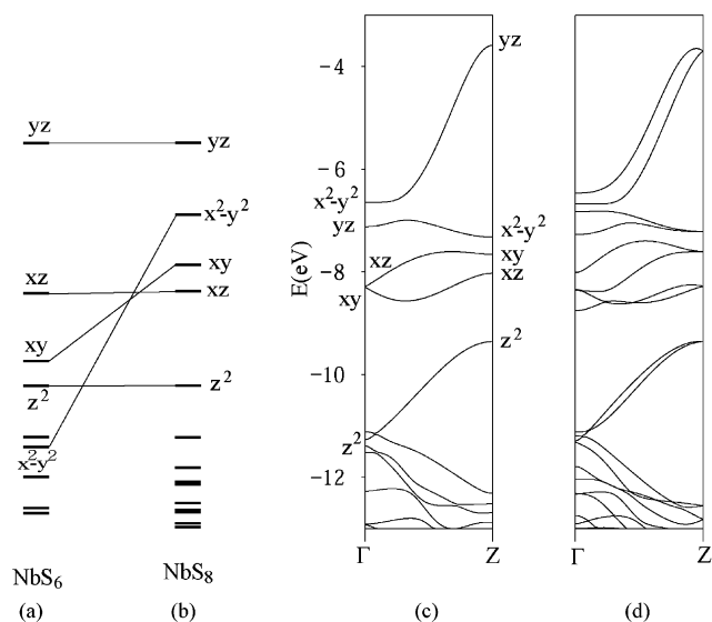
Figure 5. The MO diagrams of monomeric NbS 6 (a) and NbS 8 (b). The band structures for a single {}^1\infty[\text{NbS}_5] chain (c) and a double {}^1\infty[\text{Nb}_2\text{S}_8] chain (d).
