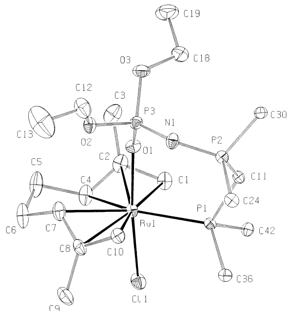
Figure 3. ORTEP-type view of the structure of the cation [\text{Ru}(\eta^3\text{-}C_{10}H_{16})\text{Cl}(\kappa^2\text{-}P,\text{O}\text{-Ph}_2\text{PCH}_2\text{P}\{\text{=NP(=O)(OEt)}_2\}\text{Ph}_2)]^+ ( 7a ) showing the crystallographic labeling scheme. Hydrogen atoms are omitted for clarity, and only the ipso -carbons of the phenyl rings of the \text{Ph}_2\text{P} groups are shown. Thermal ellipsoids are drawn at 20% probability level. Selected bond lengths (Å) and angles (deg) involving the Ru atom: Ru–C(1) = 2.227(4); Ru–C(2) = 2.304(4); Ru–C(4) = 2.309(4); Ru–C(7) = 2.265(4); Ru–C(8) = 2.297(4); Ru–C(10) = 2.232(4); Ru–C* = 2.0317(44); Ru–C** = 2.0178(42); Ru–P(1) = 2.4288(12); Ru–O(1) = 2.128(3); Ru–Cl(1) = 2.3960(13); C*–Ru–C** = 129.68(17); C*–Ru–O(1) = 88.93(16); C**–Ru–O(1) = 89.91(15); C*–Ru–Cl(1) = 88.89(14); C**–Ru–Cl(1) = 95.94(14); C*–Ru–P(1) = 114.01(14); C**–Ru–P(1) = 116.31(13); O(1)–Ru–P(1) = 91.91(8); O(1)–Ru–Cl(1) = 173.80(8); P(1)–Ru–Cl(1) = 83.69(5); Ru–P(1)–C(11) = 115.21(13); Ru–P(1)–C(36) = 119.73(14); Ru–P(1)–C(42) = 114.35(14); P(3)–O(1)–Ru = 143.89(18). C* and C** = centroids of the allyl units (C(1), C(2), C(4) and C(7), C(8), C(10), respectively).
