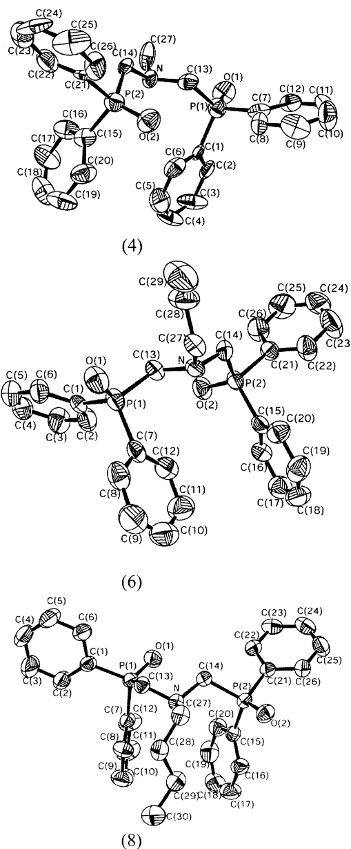
Figure 1. Perspective view of the compounds 4 , 6 , and 8 with atomic numbering scheme. Thermal ellipsoids are drawn with 50% probability level, and hydrogen atoms are omitted for clarity.
