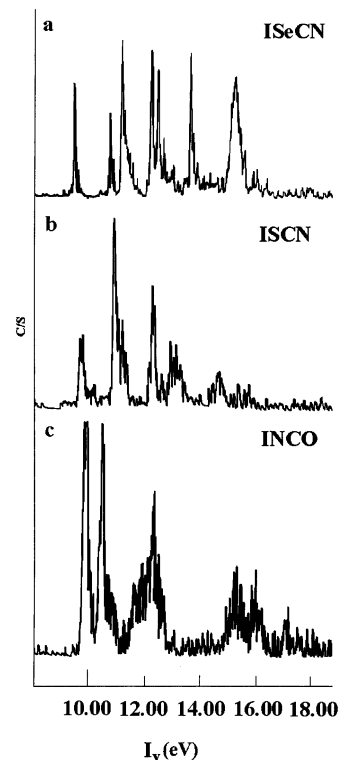
Figure 1. PE spectra of ISeCN (a), ISCN (b), and INCO (c).
