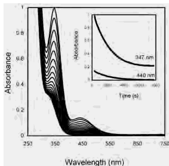
Figure 4. Spectral changes recorded during the dissociation of NO from the [\text{Fe}(\text{CN})_5\text{NO}]^{3-} complex in the presence of free cyanide: [\text{Fe}(\text{CN})_5\text{NO}]^{3-} = 3 \times 10^{-4} \text{ M} , pH 10.2 (0.05 M borate buffer), I = 0.1 \text{ M} ( \text{NaClO}_4 ), [\text{CN}^-] = 0.03 \text{ M} , T = 50.4 \text{ }^\circ\text{C} , cycle time 312 s. Inset: Kinetic traces at 440 and 347 nm, k_{\text{obs}} = 5.14 \times 10^{-4} \text{ s}^{-1} .
