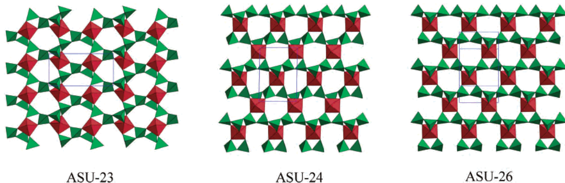
Figure 2. The oxide layer can be described as an assembly of ZrGe_5 motifs, in (left) ASU-23, (middle) ASU-24 (and ASU-25), and (right) ASU-26.
