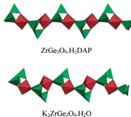
Figure 4. Comparison of the layers of umbite, projected down the b axis: (top) ZrGe_3O_9 \cdot H_2DAP and (bottom) K_2ZrGe_3O_9 \cdot H_2O .
