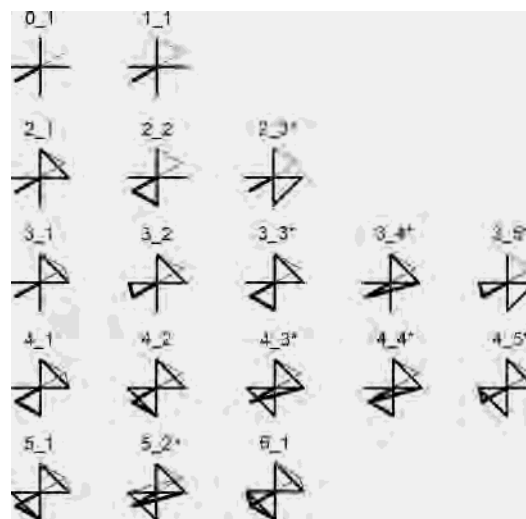
Figure 5. Combinations (18) of three-membered rings around a central octahedron have been generated; among them eight are chiral (marked with an asterisk). The most constrained arrangements have been discarded. Motif 3_2 is the motif found in the four structures ASU- n ( n = 23-26 ).
