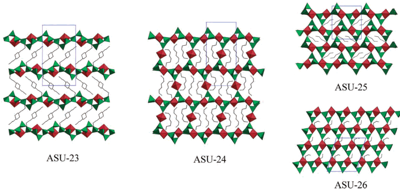
Figure 3. Stacking of layers of (left) ASU-23, (middle) ASU-24, (right-top) ASU-25, and (right-bottom) ASU-26.
