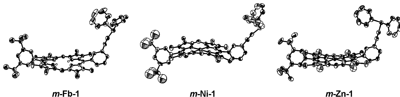
Figure 1. Molecular units of m-Fb-1 , m-Ni-1 , and m-Zn-1 , showing atomic displacement ellipsoids drawn at the 50% probability level. Hydrogen atoms and the hexyl side chains (except for the first carbon atom) have been omitted for clarity.
