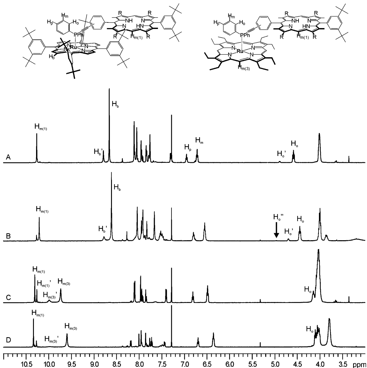
Figure 5. Low-field region of the ^1\text{H} NMR spectra of (A) [\textit{p}\text{-Fb-1/Ru-6}] , (B) [\textit{m}\text{-Fb-1/Ru-6}] , (C) [\textit{p}\text{-Fb-1/Ru-3}] , and (D) [\textit{m}\text{-Fb-1/Ru-3}] .
