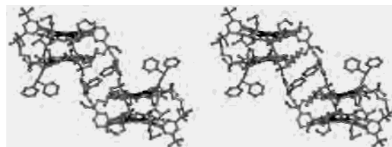
Figure 2. Stereo representation of part of the crystal packing in m-Ni-1 . Hydrogen atoms are omitted for clarity.
