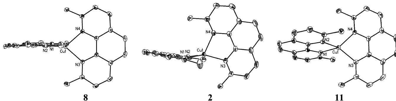
Figure 2. Geometries of \text{Cu}(\text{dmp})_2^+ cation in the complexes 2 (tetrafluoroborate acetone), 8 (tosylate), and 11 (picrate). The complexes are drawn in the plane containing the \text{N}_3\text{-C-C-N}_4 atoms.
