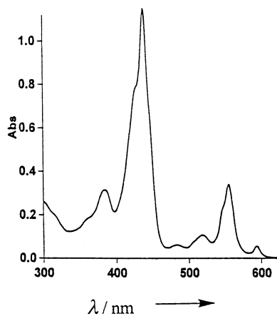
Figure 1. UV-vis spectrum of silver(III) benzocarporphyrin 15a in chloroform.
