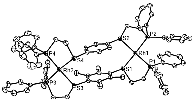
Figure 1. Thermal ellipsoid drawing of [\{1,4-(\text{Ph}_2\text{PCH}_2\text{CH}_2\text{S})_2\text{C}_6\text{H}_4\}\{1,4-(\text{Ph}_2\text{PCH}_2\text{CH}_2\text{S})_2\text{C}_6(\text{CH}_3)_4\}\text{Rh}_2]^{2+} , with 50% probability ellipsoids, in 3a showing the labeling scheme. Selected distances (Å): Rh(1)–S(2) 2.364(1), Rh(2)–S(4) 2.359(1), Rh(1)–S(1) 2.326(1), Rh(2)–S(3) 2.344(1), Rh(1)–Rh(2) 8.758, (\text{C}_6\text{H}_4)_{\text{cent}}-(\text{C}_6\text{Me}_4)_{\text{cent}} 3.591. Selected torsion angles (deg): \angle\text{S}(2)-(\text{C}_6\text{H}_4)_{\text{cent}}-(\text{C}_6\text{Me}_4)_{\text{cent}}-\text{S}(1) 5.3, \angle\text{S}(4)-(\text{C}_6\text{H}_4)_{\text{cent}}-(\text{C}_6\text{Me}_4)_{\text{cent}}-\text{S}(3) 6.6.
