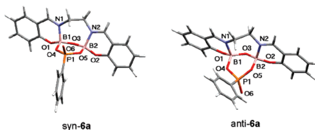
Figure 5. Calculated molecular structures of compounds syn-6a and anti-6a . Two configurations are possible for the heterotrimeric phosphonate 6a ; however, the syn conformers are thermodynamically more stable.
