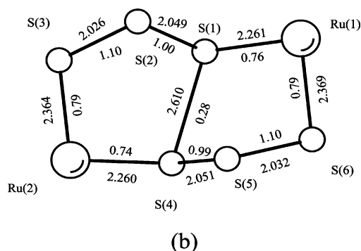
Figure 6. Bond distances (from CSD-FORBUJ) and bond orders of the Ru 2 S 6 ring in (a) [(Ru(MeCp)(PPh_3))_2(\mu_2-S_6)]^{21} and (b) [(RuCp(P(OMe)_3))_2(\mu_2-S_6)]^{22} .
