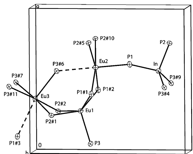
Figure 2. Partial structure of \text{Eu}_3\text{InP}_3 showing the numbering scheme and the local europium and indium environments. The anisotropic displacement ellipsoids are shown at the 90% probability level.
