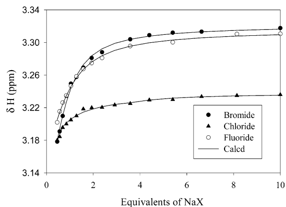
Figure 4. ^1\text{H} NMR titration curves for the aliphatic signal ( \text{NHCH}_2 ) of \text{L}^1 with \text{NaX} ( \text{X}^- = \text{F}^- , \text{Cl}^- , and \text{Br}^- ) in \text{D}_2\text{O} at 25\text{ }^\circ\text{C} and \text{pD} = 5.0 \pm 0.1 .
