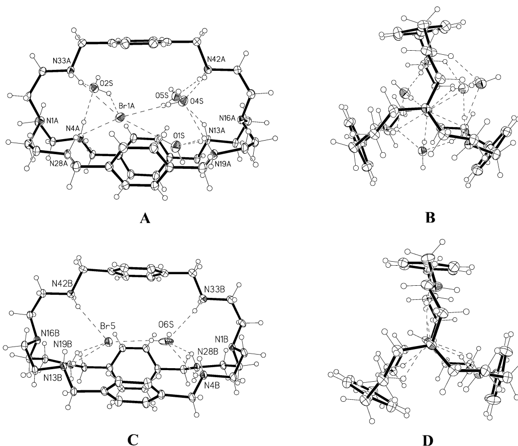
Figure 3. ORTEP drawing of [\text{H}_6\text{L}^1(\text{Br})(\text{H}_2\text{O})][\text{Br}]_5 \cdot 6.25\text{H}_2\text{O} , 3 : (A) side view showing the bromide and water molecule inside the cavity in unit A; (B) view down the three-fold axis in unit A; (C) side view showing the bromide and water molecule inside the cavity in unit B; (D) view down the three-fold axis in unit B.
