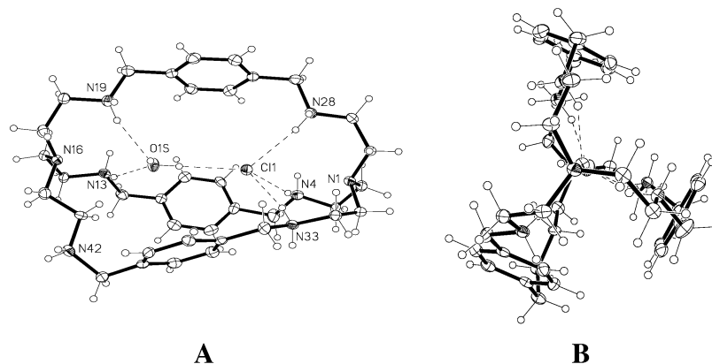
Figure 2. ORTEP drawing of [\text{H}_6\text{L}^1(\text{Cl})(\text{H}_2\text{O})][\text{Cl}]_5 \cdot 4\text{H}_2\text{O} \cdot \text{CH}_3\text{OH} , 2 : (A) side view showing the chloride and water molecule inside the cavity; (B) view down the three-fold axis.
