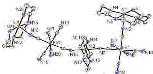
Figure 1. Crystallographic view of the asymmetric unit of 1 , H-atoms and water molecules are omitted for clarity. The inset shows the concomitant presence of meridional and facial arrangement of [\text{Fe}(\text{CN})_6]^{3-} unit.
