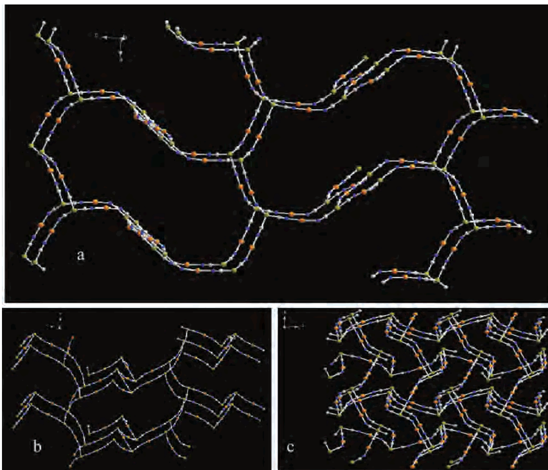
Figure 2. (a) The view of the 60 atom macrocyclic [\text{Fe}_6\text{Fe}_2\text{Ni}_4\text{Ni}_2\text{Ni}_3(\text{CN})_{20}] unit, assembled in a 2-D network and propagating along the b -axis. (b) Propagation along the a -axis. (c) Propagation along the b -axis. (The 323 ligand, terminal cyanides, and water molecules are omitted for clarity.)
