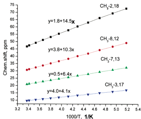
Figure 5. Curie plot for the four methyl resonances of (OMTPCrr)FeCl. The extrapolated diamagnetic shifts (assuming strict Curie behavior) are given as the constants in the linear regression of each line. As is clear from these values, the extrapolated diamagnetic shifts are within \pm 2 ppm of the expected diamagnetic shift of these methyl groups.
