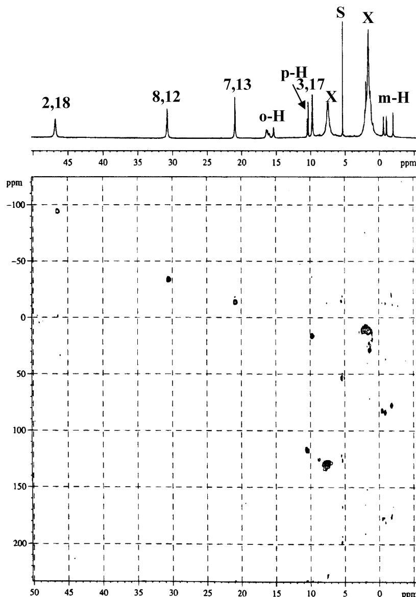
Figure 4. 1D ^1\text{H} and HMQC spectrum of (\text{OMTPCrr})\text{FeCl} , using the numbering system appropriate for describing the pyrrole- and meso -carbons to which the substituents are attached, rather than the numbering system of those substituents used for the crystal structure shown in Figure 2. The ^1\text{H} – ^{13}\text{C} correlations for the four methyl, two para -phenyl, and four meta -phenyl groups are shown; the relaxation times of the ortho -phenyl carbons are too short to allow the correlations to be detected. The ^{13}\text{C} chemical shifts of all detected HMQC crosspeaks are included in Table 2. Recorded in \text{CD}_2\text{Cl}_2 at 25 °C.
