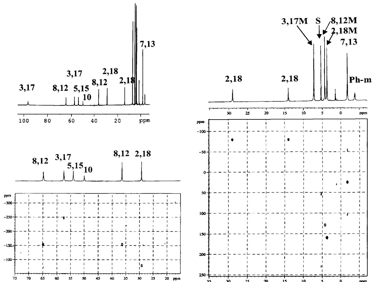
Figure 7. 1D ^1\text{H} (top left) and two expanded region HMQC spectra of (7,13-DMHECorr)FePh, showing the ^1\text{H} – ^{13}\text{C} correlations for the 7,13 methyl group and the three ethyl groups (2,18; 3,17; and 8,12). One of the 3,17- \text{CH}_2 resonances is not included in the windows used for the HMQC spectra of this figure, but its ^{13}\text{C} shift is the same as that of the other 3,17- \text{CH}_2 carbon (–250 ppm). The window of the lower-left-hand HMQC spectrum is that of the expanded region of the ^1\text{H} spectrum between 75 and 20 ppm, and that of the right-hand HMQC spectrum is of the expanded region between 35 and –5 ppm. The phenyl resonances, including those of the ortho - (–149 ppm) and para -H (–74.9 ppm) are not shown in the 1D ^1\text{H} spectrum, and no HMQC crosspeaks were observed for any phenyl-carbon resonances because of their short relaxation times. The ^{13}\text{C} chemical shifts of all detected HMQC crosspeaks are included in Table 3. Recorded in \text{CD}_2\text{Cl}_2 at 25 ^\circ\text{C} .
