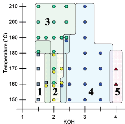
Figure 1. Composition diagram for the NiCl 2 ·6H 2 O/H 2 BDC/KOH/2,2'-bipy system. The scale on the x axis represents the molar ratio of KOH to NiCl 2 ·6H 2 O. The symbols correspond to individual reactions and the colors to specific compounds. Grey squares: 1 . Yellow circles: 2 . Green hexagons: 3 . Blue circles: 4 . Red triangles: 5 .
