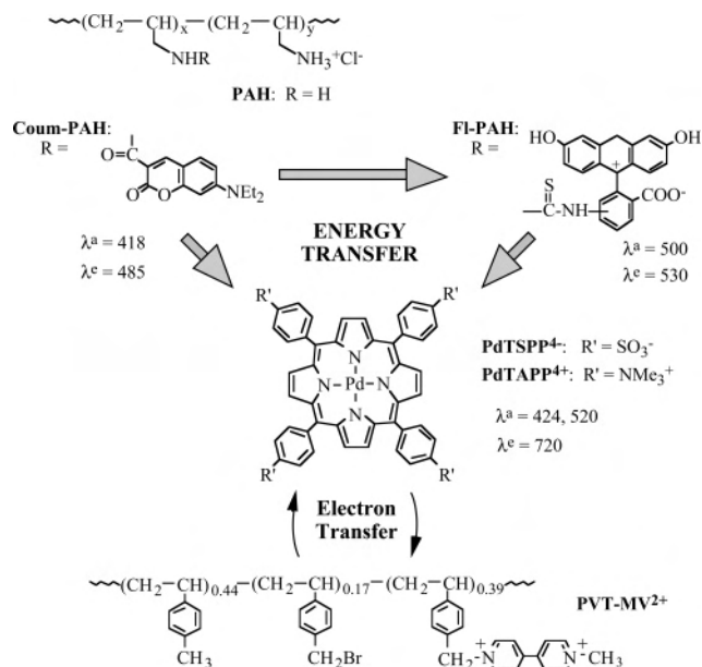
Figure 6. Molecular structures and energy- and electron-transfer pathways (indicated by arrows) for the energy “antenna” polymers, Coum-PAH and Fl-PAH; the photosensitizers, PdTAPP 4+ and PdTSPPP 4+ ; and the electron-acceptor polymer, PVT-MV 2+ .
