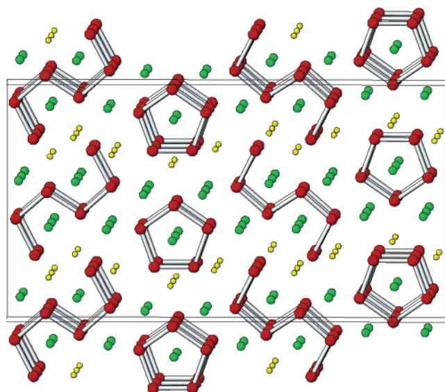
Figure 5. View of the structure of \text{Li}_5\text{Ca}_7\text{Sn}_{11} along the a -axis ( c is horizontal; Li, yellow; Ca, green). Flat zigzag hexamers of tin are stacked on top of each other to form columns along a that are parallel to the columns of stacked pentagonal rings of tin. Both the rings and the hexamers alternate with calcium cations within the columns.
