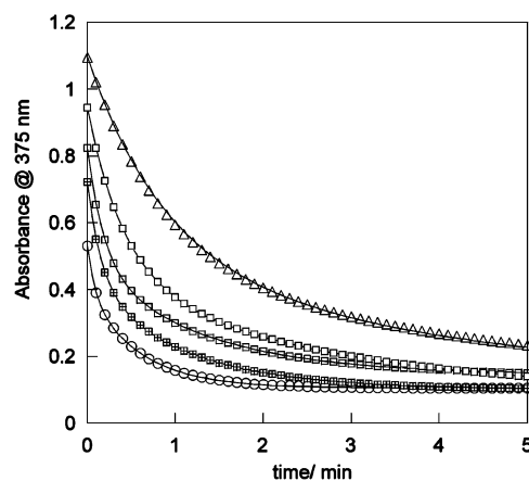
Figure 3. Absorbance–time curves for the reaction of complex 1 with MeI ( 0.053\text{--}0.53\text{ M} ; [MeI] increases reading downward) in benzene at 25^\circ\text{C} . The solid lines were obtained by fitting the (A, t) data into eq 2.
