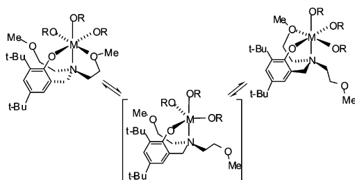
Scheme 2. Proposed Equilibration Processes for the Alkoxido Complexes 1 and 2
