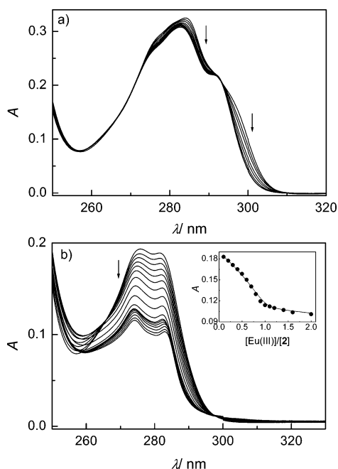
Figure 1. Changes in the absorption spectra of (a) 1 and (b) 2 upon titration with Eu(III) triflate ( [1] = 7.65 \times 10^{-5} M, [2] = 6.89 \times 10^{-5} M). The inset shows the titration curve at \lambda_{\text{obs}} = 279 nm and the corresponding fit.
