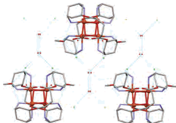
Figure 12. Packing of hydrogen-bonded subunits parallel to the crystallographic c axis (viewed from the a axis) in [\{Cu_2(OH)_2(GADACE)\}_2]Cl_4 \cdot 2MeOH \cdot 6H_2O , 6 . Color codes as in Figure 3.
