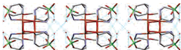
Figure 8. Hydrogen-bonded chain in 5 viewed along the crystallographic a axis. Color codes as in Figure 3.
