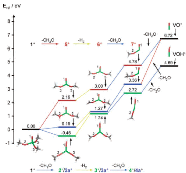
Figure 4. Calculated energetics (in eV) from the cation 1 + to the quasi-terminal fragments VO + and VOH + . Also see Table 5.
