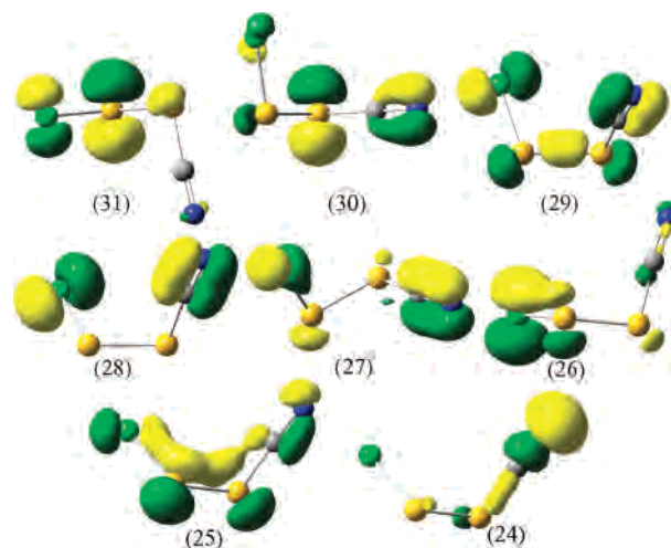
Figure 3. Characters of the first eight highest occupied molecular orbitals for CISSCN.
