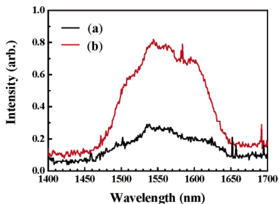
Figure 5. Near-IR–fluorescence spectra of (a) 1a and (b) 2a excited at 808 nm by a LD.
