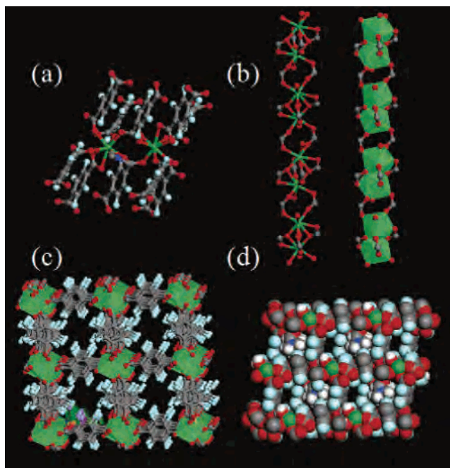
Figure 2. Structure of 2 showing (a) the coordination geometry of the binuclear \text{Er}_2(\text{BDC-F}_4)_3(\text{DMF})(\text{H}_2\text{O}) fragment, (b) a 1D infinite secondary building unit with ball-and-stick representation (left) and with Er atoms shown as polyhedra (right), (c) a 3D MOF viewed along the 1D \text{Er}_2(\text{CO}_2)_6 rod (DMF and \text{H}_2\text{O} molecules are omitted for clarity), and (d) a space-filling representation viewed along the a axis (uncoordinated DMF molecules are omitted for clarity; Er, light green; F, light cyan; N, blue; O, red; C, gray).
