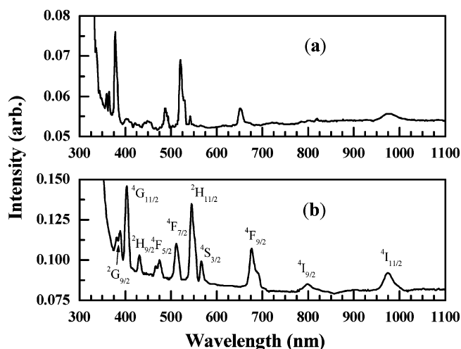
Figure 4. UV–vis–near-IR absorption spectra of (a) 1 and (b) 2 , respectively.
