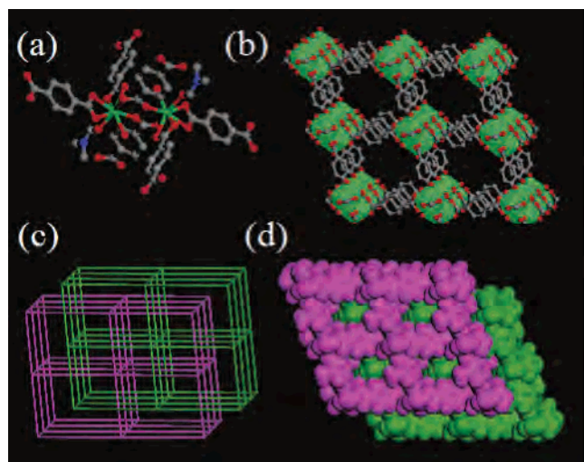
Figure 1. Structure of 1 showing (a) the coordination geometry of the secondary building unit of a Er 2 (BDC) 3 (DMF) 2 (H 2 O) 2 cluster, (b) its primitive cubic α-Po net (H atoms are omitted for clarity; Er, light green; N, blue; O, red; C, gray), (c) a schematic illustration of the doubly interpenetrating frameworks in purple and green [center of the Er 2 (BDC) 3 (DMF) 2 (H 2 O) 2 cluster as the Po node], and (d) its corresponding space-filling representation indicating the formation of a condensed structure.
