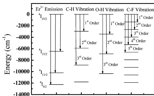
Figure 6. Schematic representation of the vibrational quenching of the {}^4\text{I}_{13/2} emission of \text{Er}^{3+} by the vibrational modes of CH, OH, and CF functional groups.
