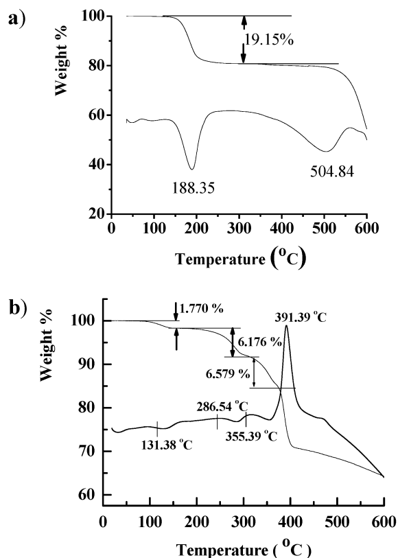
Figure 3. TGA–DSC diagrams of (a) 1 and (b) 2 .
