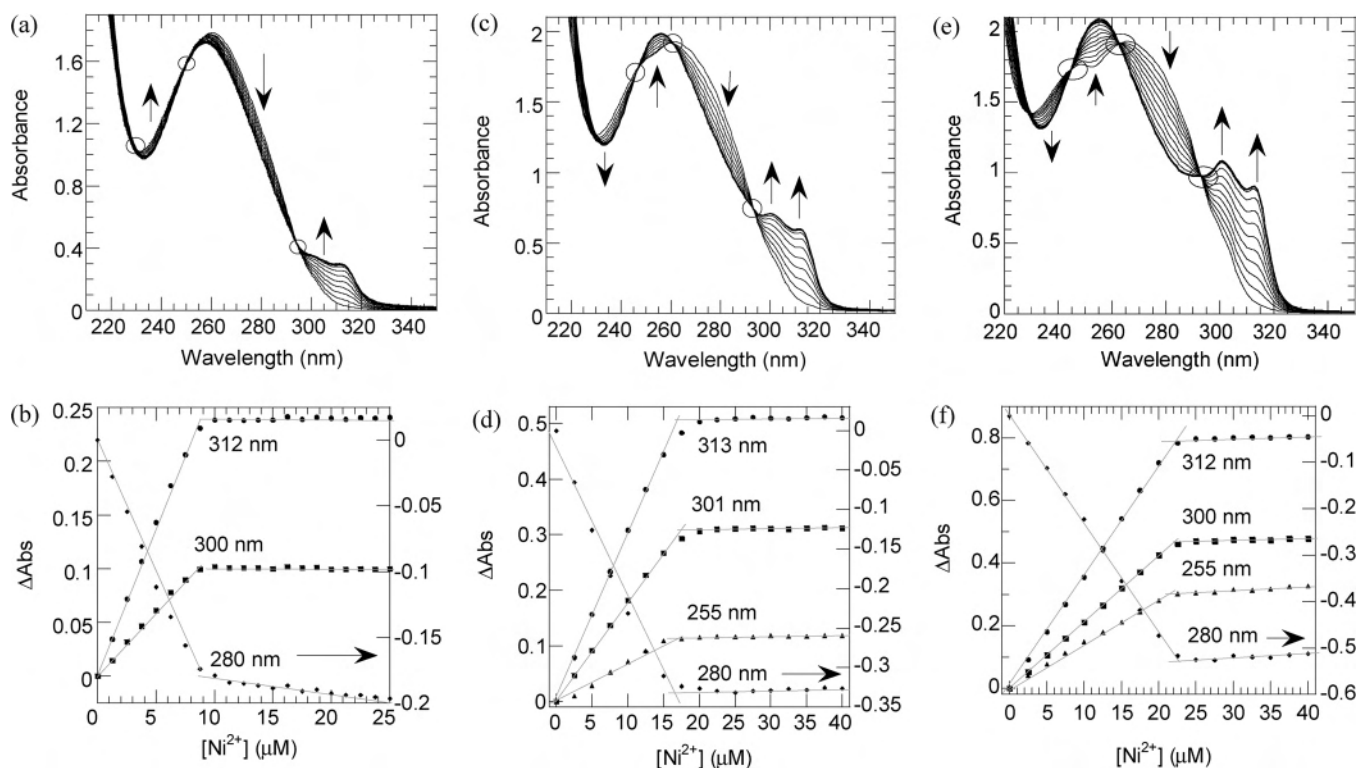
Figure 6. Spectrophotometric titration of 20 \mu\text{M A}^9 (a and b), 20 \mu\text{M A}^{5,6} (c and d), and 20 \mu\text{M A}^{5,6,7} (e and f) in pH 7, 10 mM sodium phosphate buffer with \text{Ni}^{2+} .
