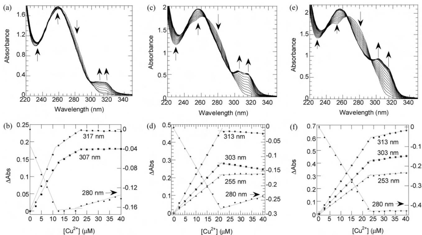
Figure 7. Spectrophotometric titration of 20 \mu\text{M A}^9 (a and b), 20 \mu\text{M A}^{5,6} (c and d), and 20 \mu\text{M A}^{5,6,7} (e and f) in pH 7, 10 mM sodium phosphate buffer with \text{Cu}^{2+} .
