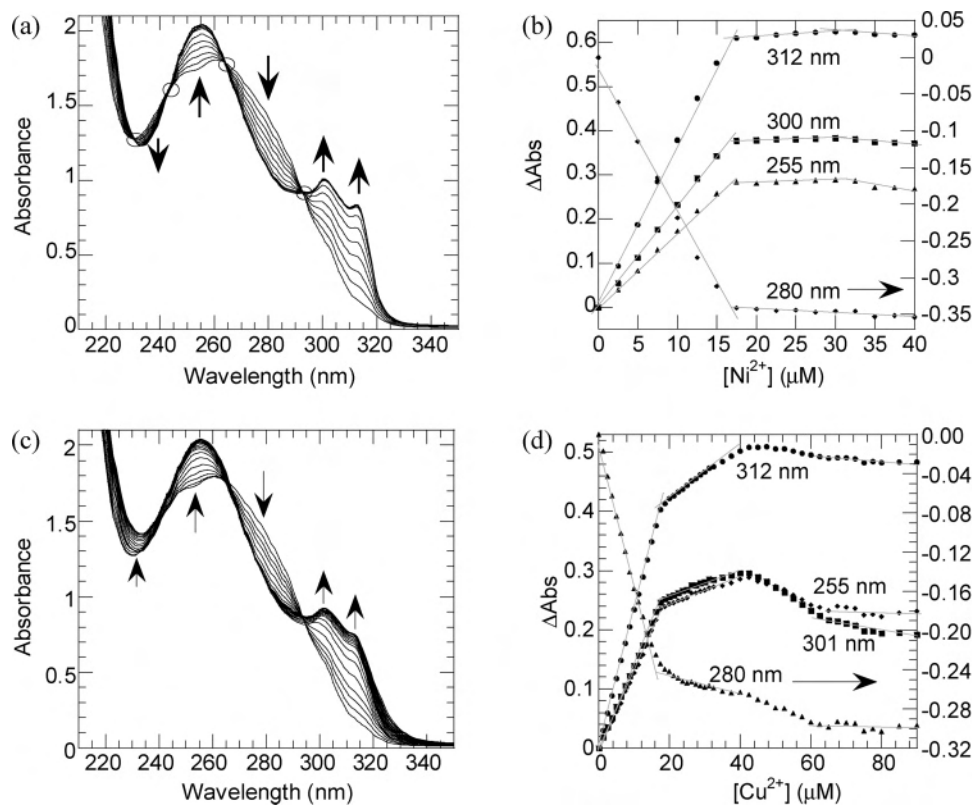
Figure 5. Titration of 10 \mu\text{M} \{\text{AB}\}^{5,6,7} in pH 7, 10 mM sodium phosphate buffer with \text{Ni}^{2+} (a and b) and \text{Cu}^{2+} (c and d). See Figure S4 for spectral changes at successive \text{Cu}^{2+} concentration regimes.
