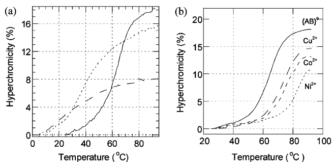
Figure 1. Melting curves measured for (a) 5 μM { AB } 9 (solid line), { AB } 5,6 (dotted line), and { AB } 5,6,7 (dashed line) in the absence of transition metal ions and (b) 5 μM { AB } 9 duplexes in the absence and presence of 1 equiv of Ni 2+ , Cu 2+ , or Co 2+ . Solutions were prepared in pH 7, 10 mM sodium phosphate buffer.
