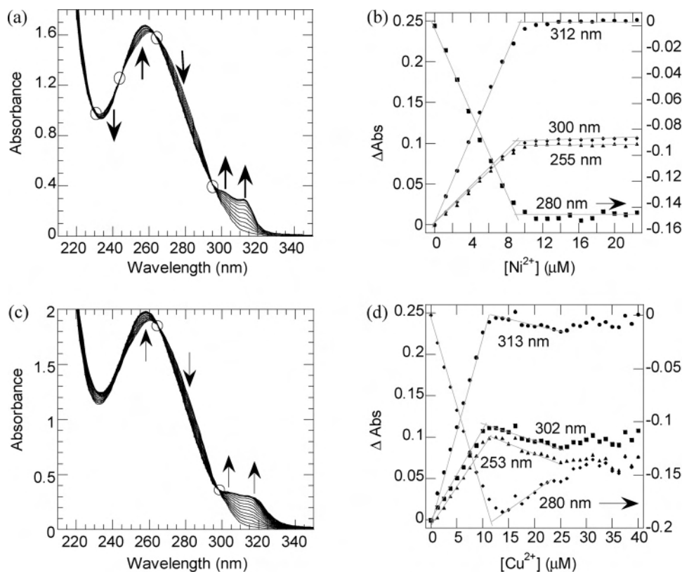
Figure 3. Spectrophotometric titration of 10 \mu\text{M} \{\text{AB}\}^9 solutions in pH 7, 10 mM sodium phosphate buffer with \text{Ni}^{2+} (a and b) or \text{Cu}^{2+} (c and d).
