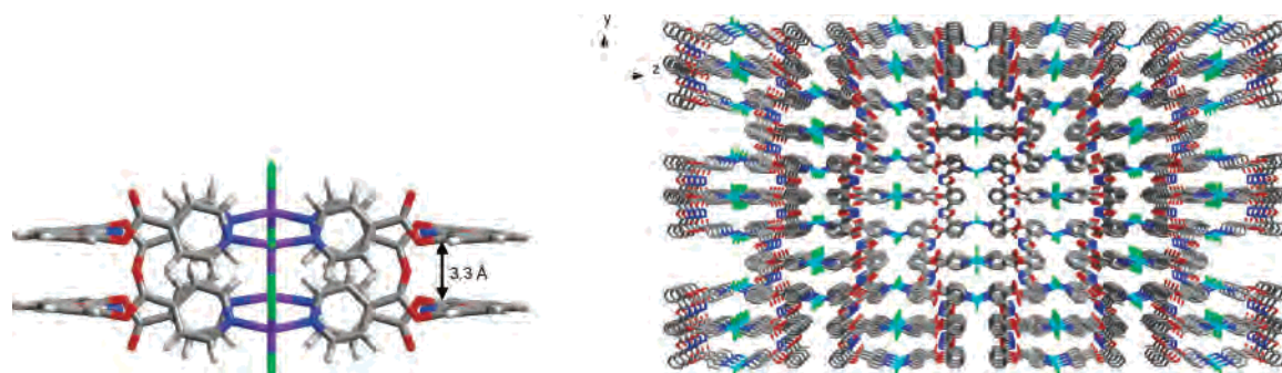
Figure 10. Inter-ring \pi-\pi (3.3 Å) interaction in the tetranuclear double macrocycles (left) and crystal packing (right) of 5.
