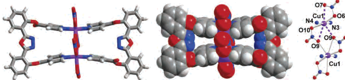
Figure 5. Stick (left), space-filling model (middle), and copper coordination sphere (right) of compound 3 .
