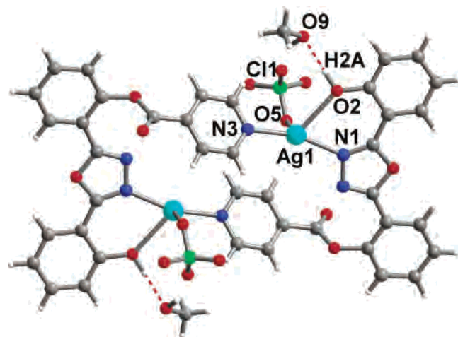
Figure 3. Molecular structure of 2.
