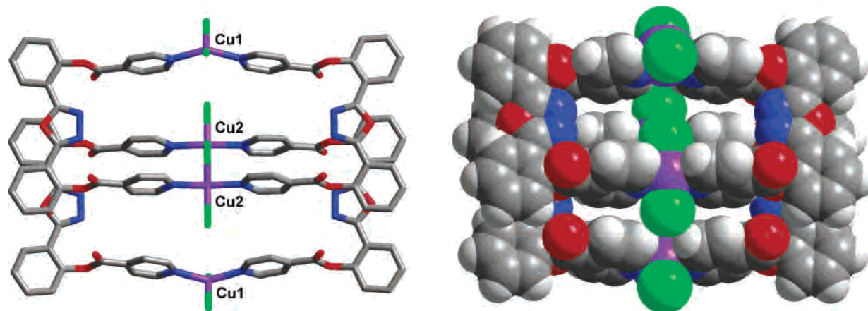
Figure 9. Tetranuclear double macrocycles in 5.
