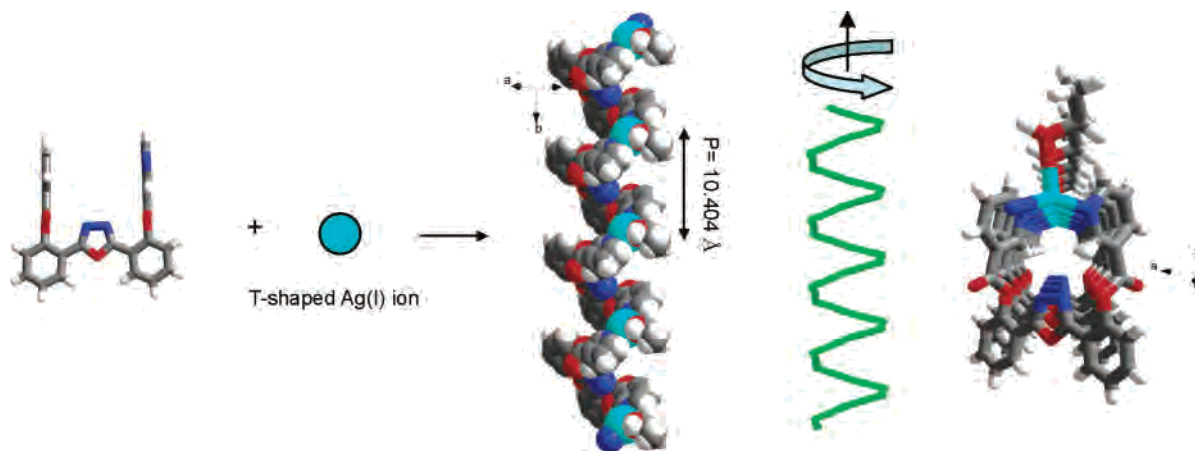
Figure 15. Design for the molecular helical chain from a combination of the silver(I) ion and the “Σ-shaped” spacer (side and top views).
