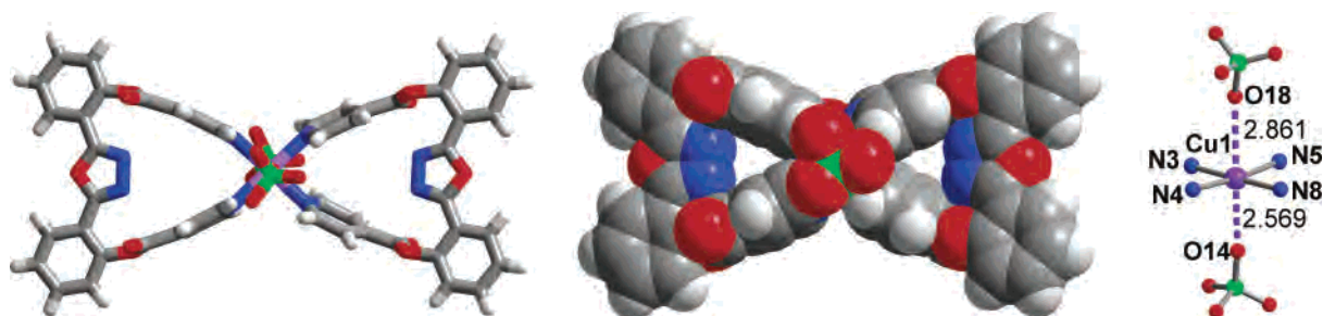
Figure 7. Stick (left), space-filling model (middle), and copper coordination sphere (right) of 4.
