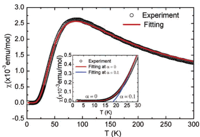
Figure 1. Temperature dependence of the magnetic susceptibility of [\text{Cu}(\text{OH})(\text{C}_5\text{H}_4\text{NCO}_2)\cdot\text{H}_2\text{O}] from 2 to 300 K. The open circles represent the data after subtraction of the impurity contribution, while the red line is the result of fitting to the spin dimer equation. For comparison, the blue line shows the alternating-chain model at \alpha = 0.1 (inset).
