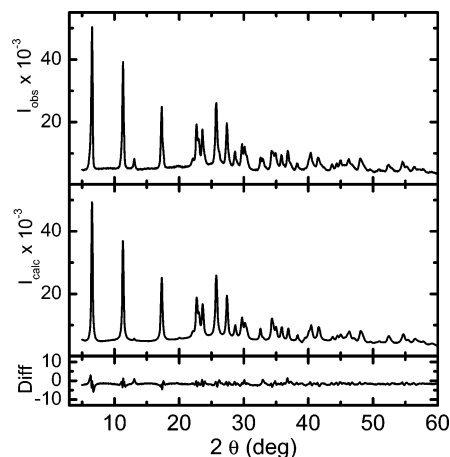
Figure 2. Experimental and calculated X-ray powder pattern for 2 ( R_1 = \text{Me} , R_2 = \text{Ph} ).
