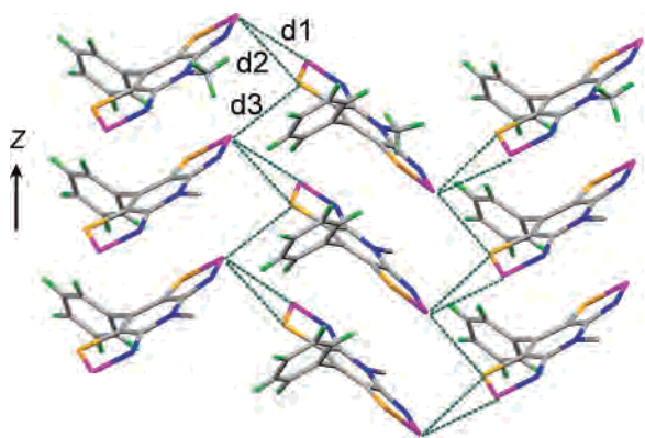
Figure 4. Herringbone \pi -stacking of 2 ( R_1 = \text{Me} , R_2 = \text{Ph} ). Intermolecular contacts d1–d3 are defined in Table 3. (Color code: Se, pink; S, yellow; N, blue.)
