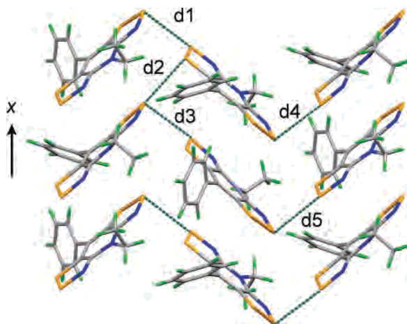
Figure 6. \pi -Stacking of 1 ( R_1 = \text{Et} , R_2 = \text{Ph} ). Intermolecular contacts d1–d5 are defined in Table 3. (Color code: S, yellow; N, blue.)
