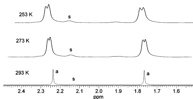
Figure 3. Selected region of the variable-temperature ^1\text{H} NMR spectra (300 MHz, Tol- d_8 ) of 4 . Descriptors a and s refer, respectively, to the \text{CH}_3 pyrazolyl groups of 4 and the residual solvent resonances (Tol- d_8 ).
