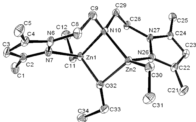
Figure 8. Solid-state structure of 12 (ellipsoids drawn at the 50% probability; hydrogen atoms omitted for clarity). Selected bond lengths (Å) and angles (deg): Zn(1)—C(11), 1.9954(19); Zn(1)—O(32), 2.0214(17); Zn(1)—N(10), 2.0732(17); Zn(1)—N(7), 2.1010(16); Zn(2)—N(10), 2.0595(18); Zn(2)—N(26), 2.1144(16); Zn(2)—O(32), 2.0087(15); Zn(2)—C(30), 1.9993(19); C(11)—Zn(1)—O(32), 122.08(7); C(11)—Zn(1)—N(7), 117.09(8); O(32)—Zn(1)—N(10), 86.08(6); Zn(1)—O(32)—Zn(2), 94.22(6); Zn(1)—N(10)—Zn(2), 91.20(6); N(10)—Zn(2)—O(32), 86.77(6).
