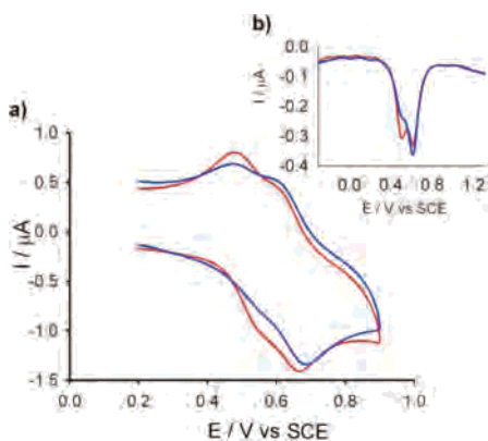
Figure 5. (a) Evolution of cyclic voltammogram of free ligand 5 (1 mM) (red) until the formation of the complex 5 ·Cd 2+ (blue) in \text{CH}_2\text{Cl}_2/\text{CH}_3\text{CN} (3/2) using [( n -Bu) 4 N]ClO 4 as supporting electrolyte scanned at 100 mV s -1 . (b, inset) Evolution of DPV of free ligand 5 (1 mM) (red) until the formation of the complex 5 ·Cd 2+ (blue) in \text{CH}_2\text{Cl}_2/\text{CH}_3\text{CN} (3/2) using [( n -Bu) 4 N]ClO 4 as supporting electrolyte scanned at 100 mV s -1 .
