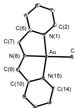
Figure 4. View of the structure of complex 5a .
