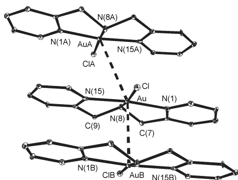
Figure 5. Packing of the [\text{AuCl}(\text{BPMA}-\text{H})]^+ ions in complex 5b . Symmetry operators: A, -x + 1, -y + 2, -z + 2 ; B, -x + 2, -y + 2, -z + 2 .
