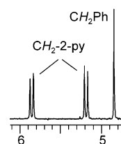
Figure 2. Methylene region of the 1 H NMR spectrum (400 MHz, CD 3 -NO 2 solution) of complex 3 , showing the diastereotopic nature of the CH a H b -2-py protons.
