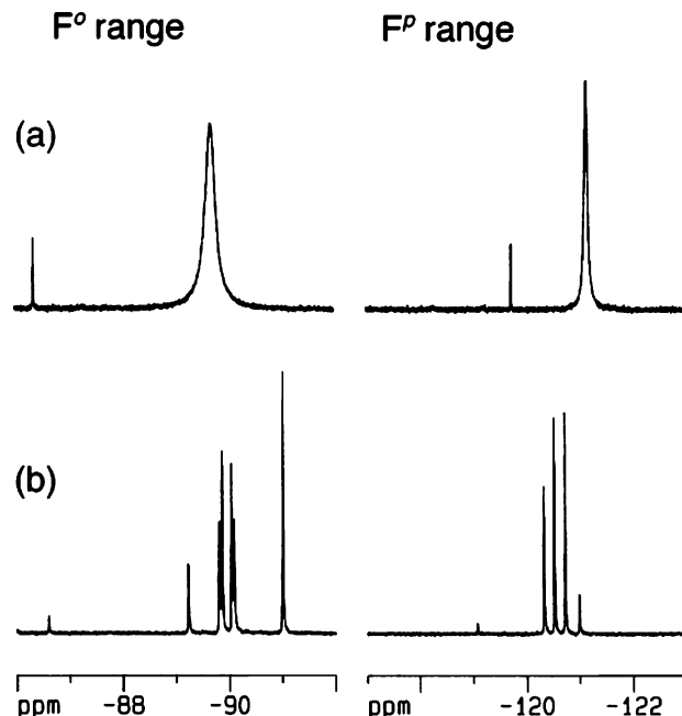
Figure 1. 19 F NMR spectra of a solution of trans -[NiRf 2 (SbPh 3 ) 2 ] ( 1a ) in wet (CD 3 ) 2 CO at 293 K (a) and 217 K (b).
