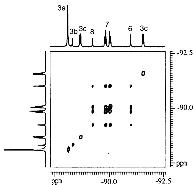
Figure 4. ^{19}\text{F} EXSY experiment in the F_0 region for complex 3a in wet (\text{CD}_3)_2\text{CO} at 217 K ( t_m = 0.5 s). The cross-peaks only correlate signals of 6 , 7 , and 8 .
