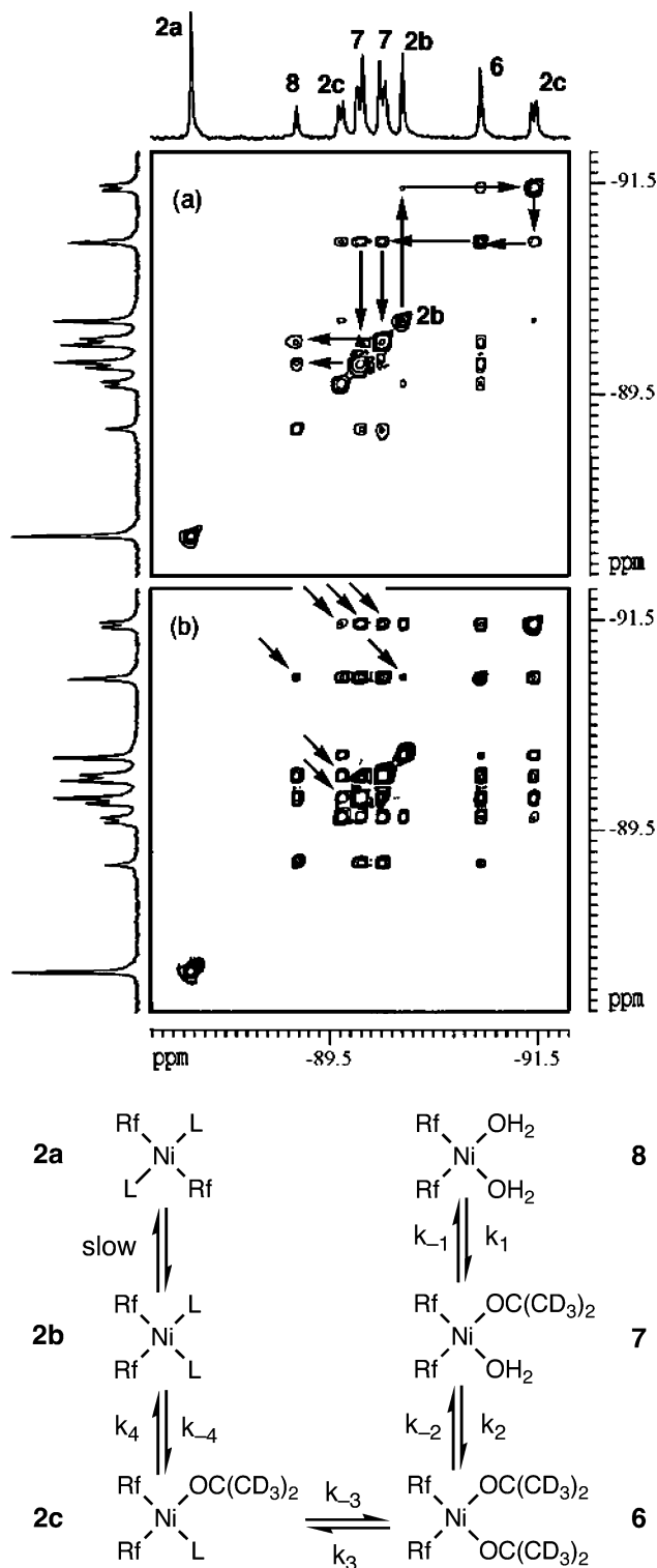
Figure 3. ^{19}\text{F} EXSY experiments in the \text{F}^o region of a solution of complex 2a in wet (\text{CD}_3)_2\text{CO} at 217 K ((a) t_m = 0.15 s, (b) t_m = 0.45 s) and scheme of the exchange processes between the different species formed. Arrows in (b) indicate the cross-peaks due to indirect exchanges ( 2b - 6 , 2c - 7 , 6 - 8 , and the intramolecular exchange of the two nonequivalent fluoroaryls groups in 2c ).
