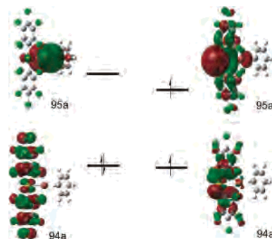
Figure 4. Molecular orbital diagrams for the ground state S_0 (left) and the lowest triplet excited state T_1 (right).
