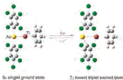
Figure 3. DFT-optimized structures for the singlet ground state and the lowest triplet excited state.
