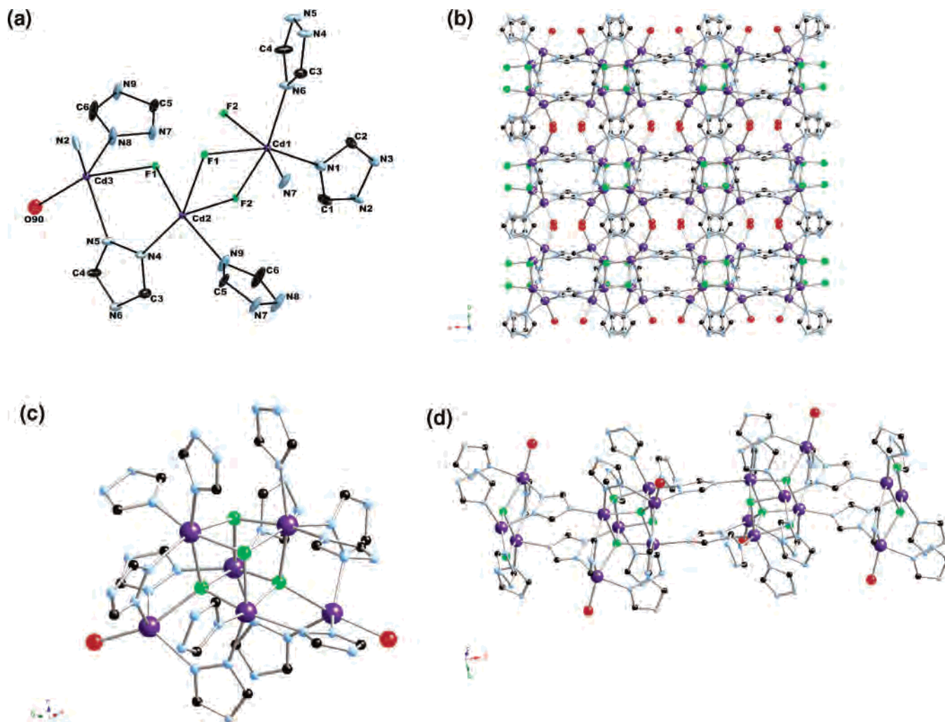
Figure 6. (a) View of the structure of [\text{Cd}_3(\text{trz})_3\text{F}_2(\text{OH})]\cdot 3\text{H}_2\text{O} ( 5\cdot 3\text{H}_2\text{O} ), showing the atom-labeling scheme and 50% thermal ellipsoids. (b) View of the three-dimensional structure of 5 in the ab -plane. (c) Hexanuclear cadmium building block of 5 , showing the \{\text{Cd}_4\text{F}_4\} core. (d) Chain of hexanuclear clusters linked through triazolate bridges.
