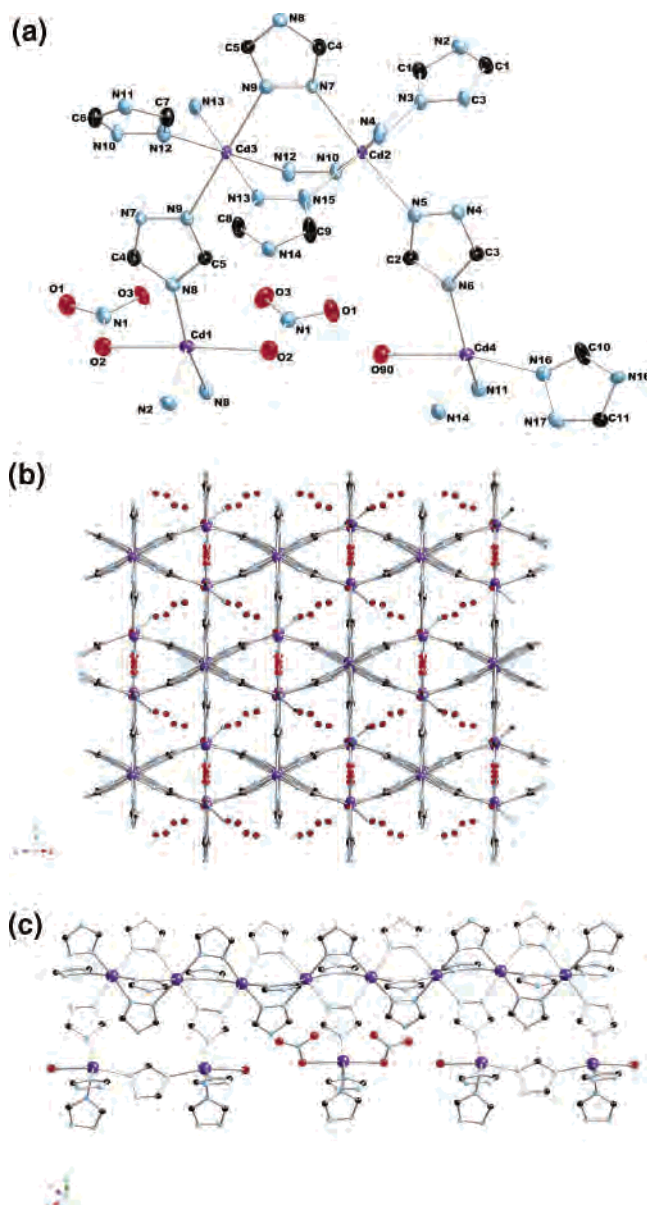
Figure 10. (a) ORTEP representation of the structure of [\text{Cd}_3(\text{trz})_5(\text{NO}_3)(\text{H}_2\text{O})]\cdot\text{H}_2\text{O} ( 9 · \text{H}_2\text{O} ), showing the atom-labeling scheme and 50% thermal ellipsoids. (b) View of the three-dimensional structure of 9 . (c) \{\text{Cd}(\text{trz})_3\}_n^{n-} chain of 9 and one set of trigonal bipyramidal and binuclear \{\text{Cd}_2(\text{trz})_7(\text{H}_2\text{O})_2\}^{3-} sites that connect the chain to neighboring chains.
