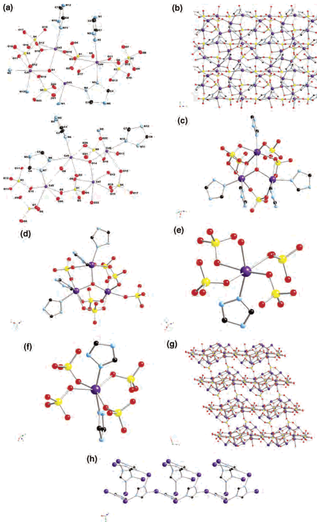
Figure 11. (a) Atom-labeling scheme and 50% thermal ellipsoids for the structure of [Cd_8(trz)_4(OH)_2(SO_4)_5(H_2O)] ( 10 ). (b) View of the three-dimensional structure of 10 in the bc -plane. (c, d) Two \eta^3 -OH-bridged cadmium triads that are observed as secondary building units of 10 . (e) Aqua-ligated \{CdNO_5\} site of 10 . (f) "Isolated" \{CdN_2O_4\} site. (g) Three-dimensional cadmium sulfate substructure of 10 . (h) One-dimensional cadmium-triazolate substructure of 10 .
