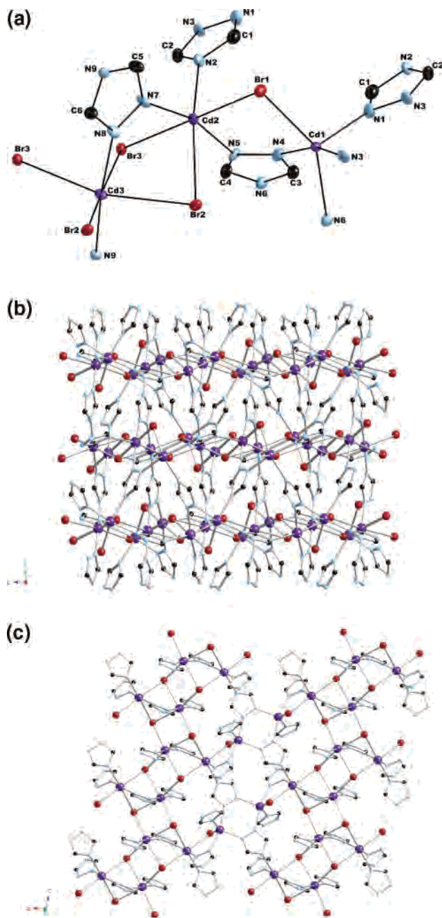
Figure 8. (a) ORTEP representation of the structure of [\text{Cd}_3(\text{trz})_3\text{Br}_3] ( 7 ), showing the atom-labeling scheme and 50% thermal ellipsoids. (b) View of the three-dimensional structure of 7 in the bc -plane. (c) Network substructure of 7 in the ac -plane showing the three cadmium environments and their linking through triazolate and bromine bridges.
