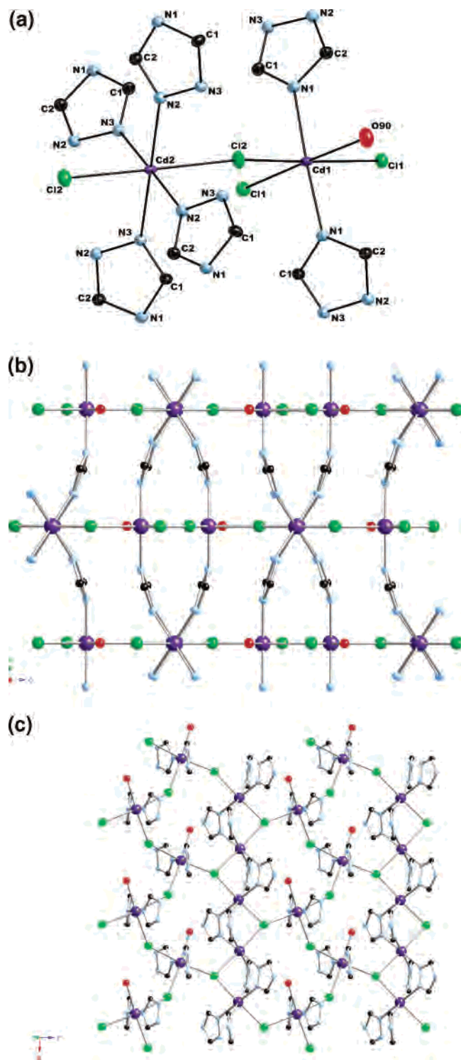
Figure 7. (a) Atom-labeling scheme and 50% thermal ellipsoids for the structure of [\text{Cd}_2(\text{trz})_2\text{Cl}_2(\text{H}_2\text{O})] ( 6 ). (b) View of the three-dimensional structure of 6 in the bc -plane. (c) View of the structure of 6 in the ac -plane, showing the \{\text{Cd}(\text{trz})_2\text{Cl}\}_n^{n-} chains running parallel to the a -axis.
